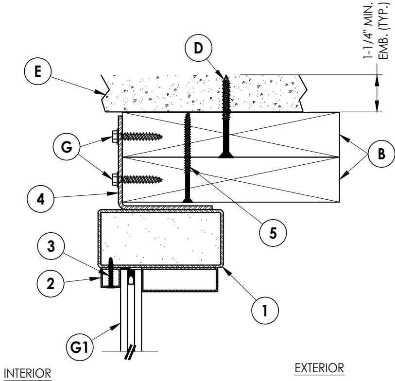
1 2 VERTICAL CROSS SECTION
